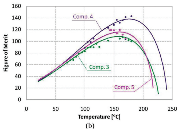
FIGURE 3 Temperature dependent figure of merit of (a) short alkyl chain NCS-phenyltolanes and (b) different alkyl chain of the same rigid core homologues.
