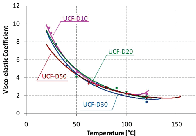
FIGURE 5 Temperature dependent visco-elastic coefficient of UCF-D systems.
