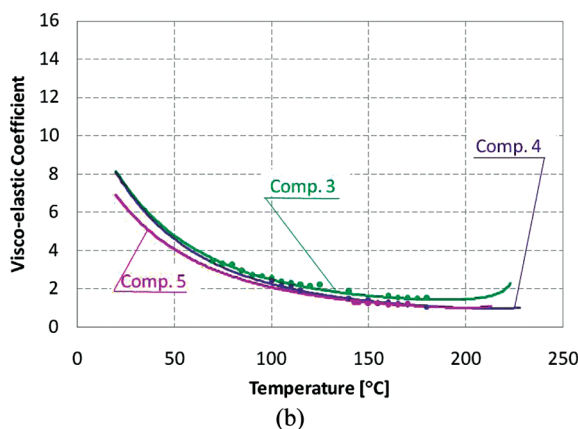
FIGURE 2 Temperature dependent visco-elastic coefficient of (a) short alkyl chain NCS-phenyltolanes and (b) different alkyl chain of the same rigid core homologues.
