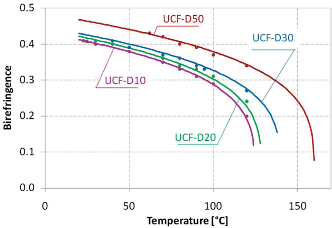
FIGURE 4 Temperature dependent birefringence of UCF-D systems.
